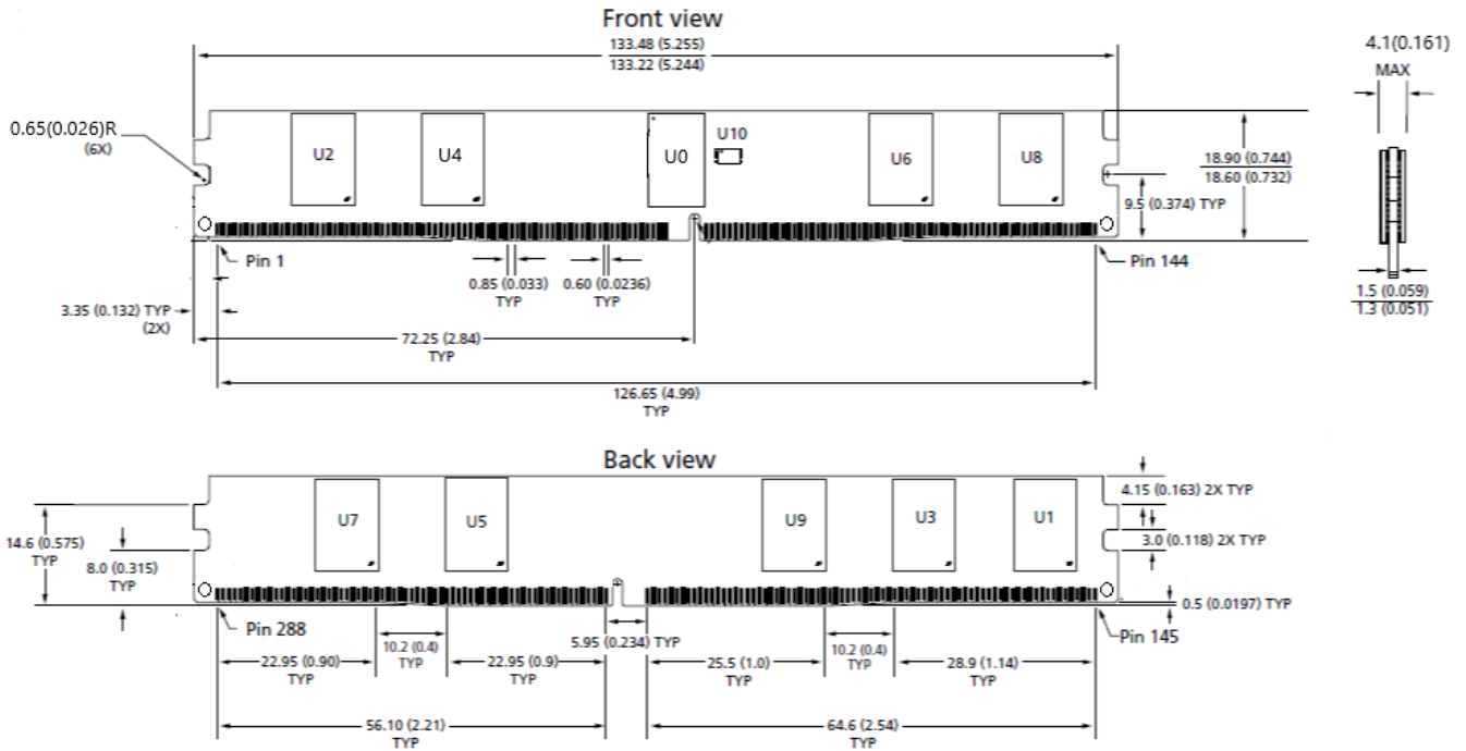
Figure 2 - Package Dimensions_SCC16GP03H2F1V-32AA
