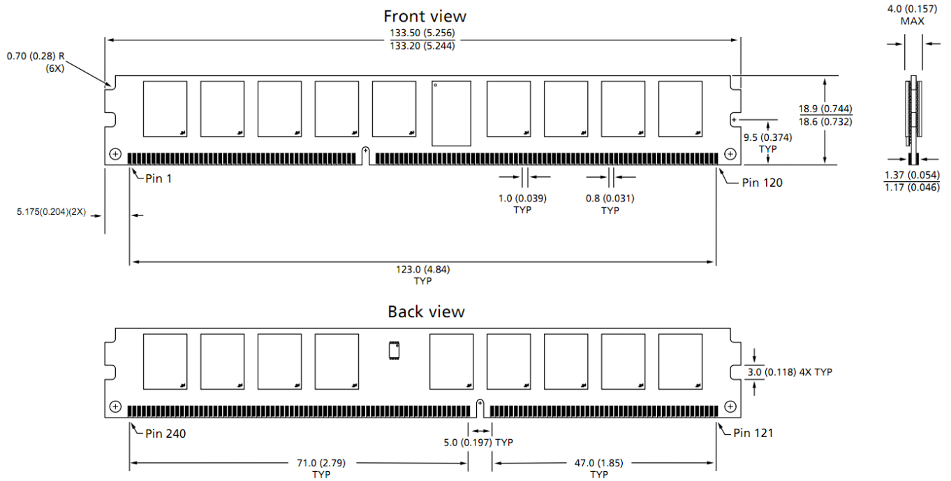
Figure 1 - Package Dimensions_ HXMSH8GP13A2F1V-16K
