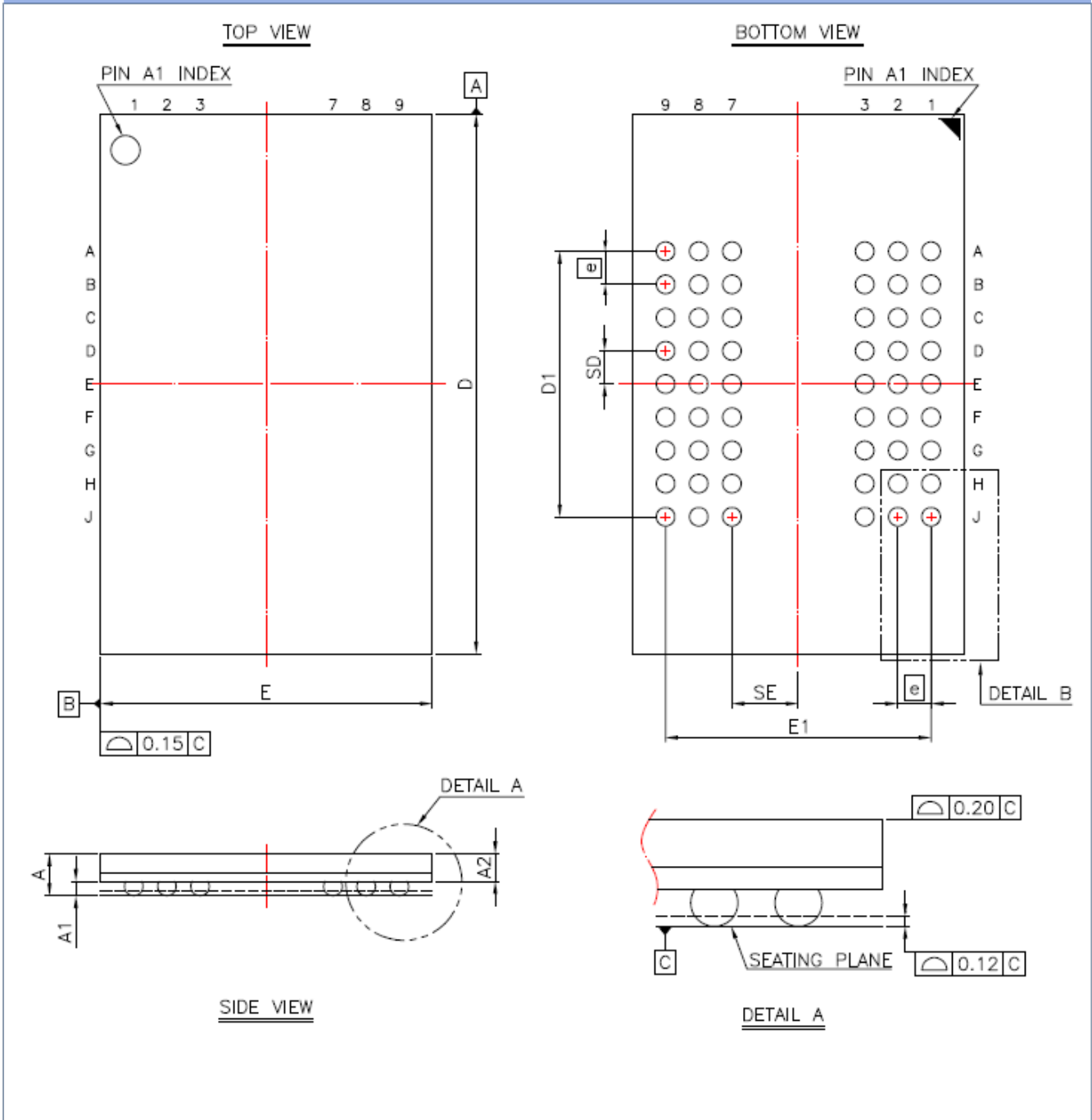
FIGURE 5 Package OutlineFBGA54
