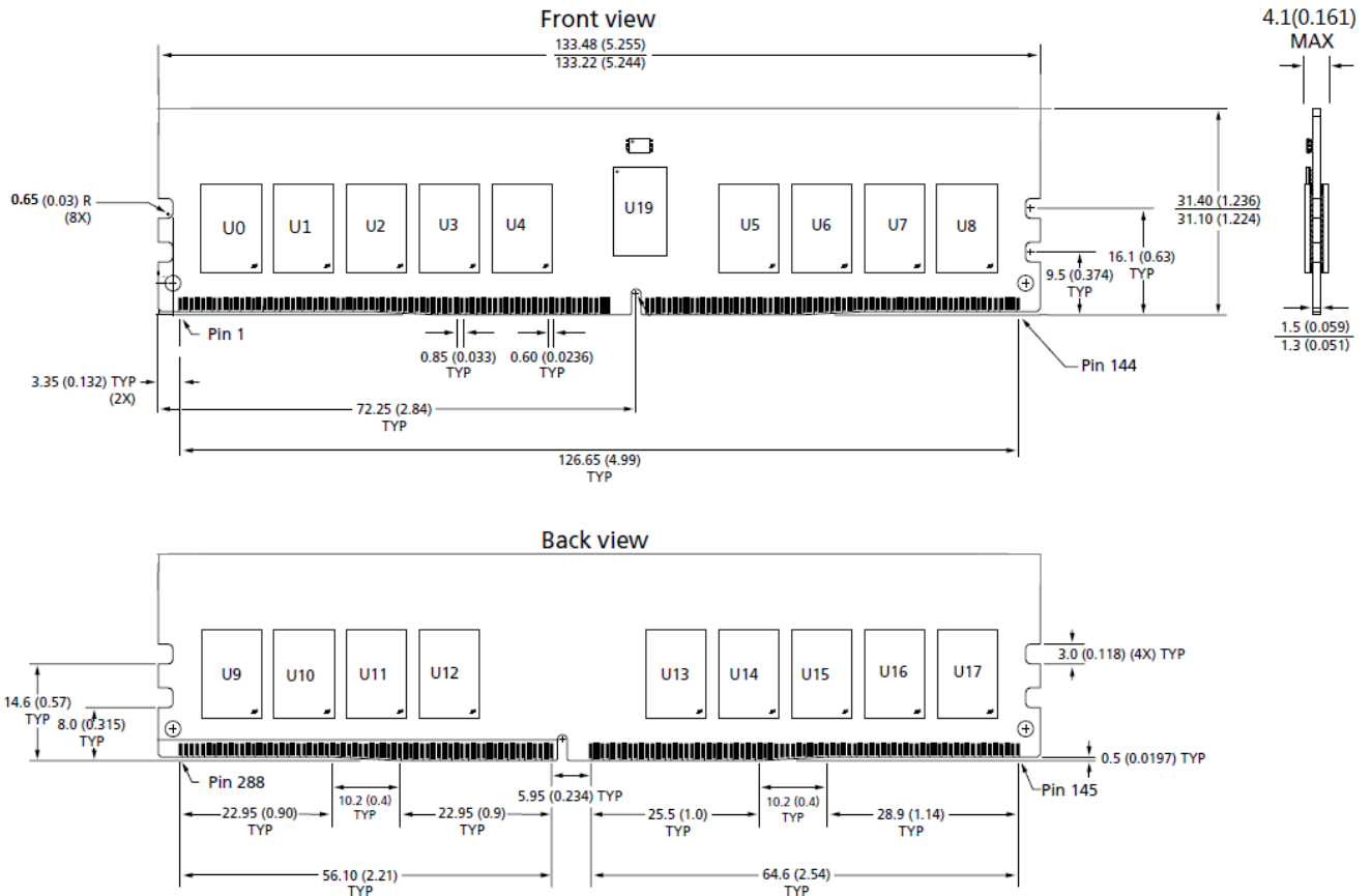
Figure 3 - Package Dimensions_SCC32GP02H2F1C-32AA
