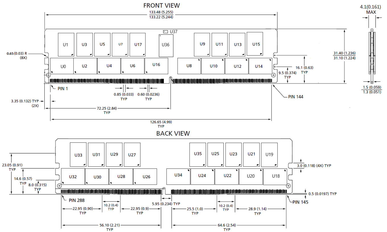
Figure 4 - Package Dimensions_SCC64GP12H2F1C-32AA
