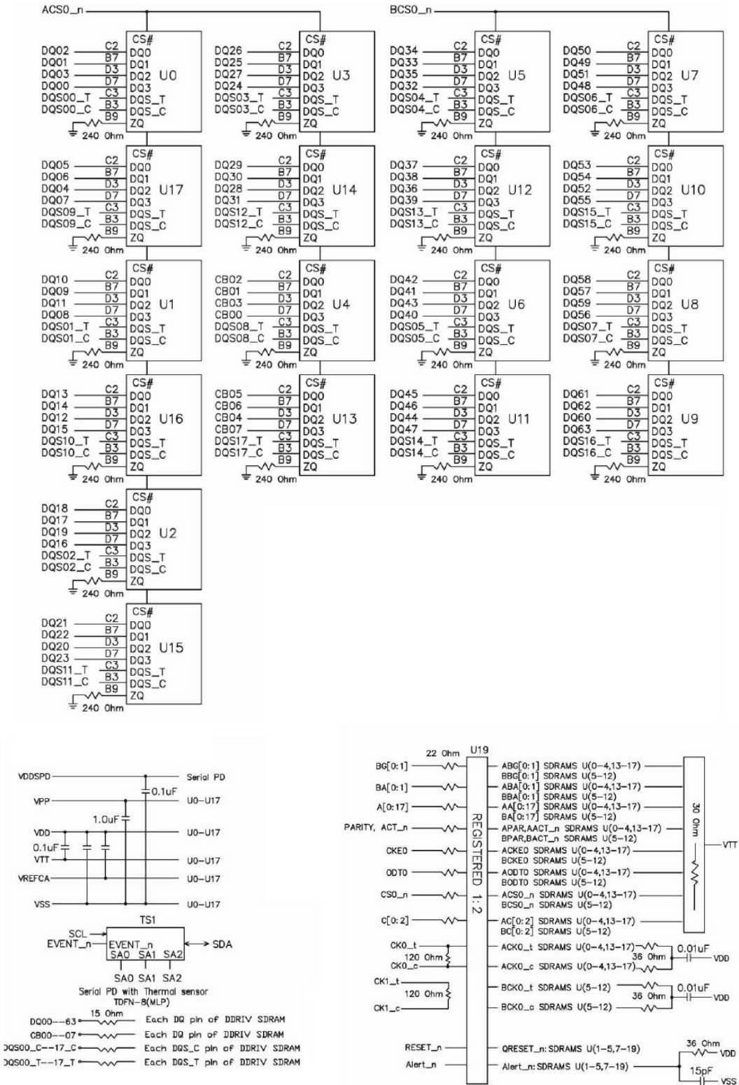
Figure 1 - Function Block Diagram_SCC32GP02H2F1C-32AA
