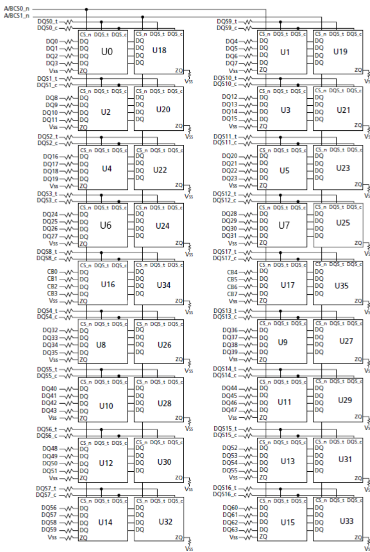
Figure 2 - Function Block Diagram_SCC64GP12H2F1C-32AA
